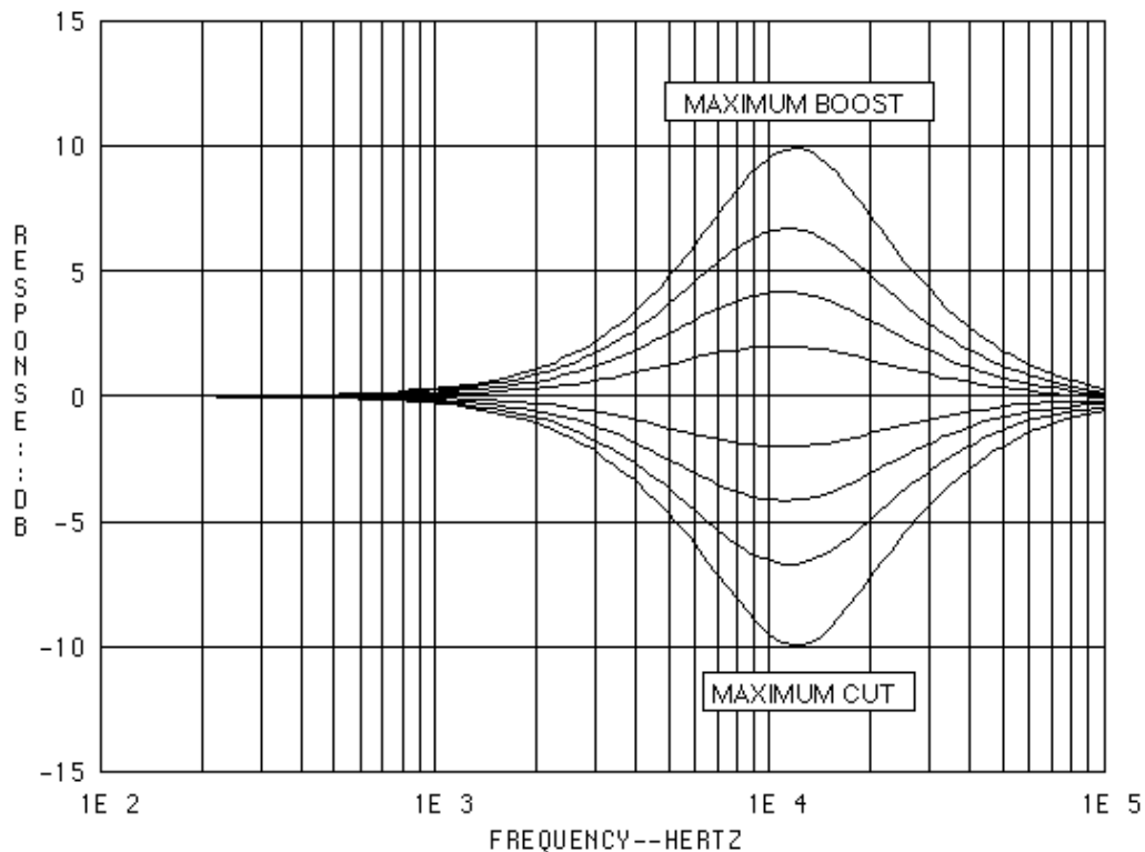
Figure 6. Treble Control Frequency Response
